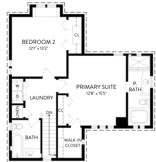
UPPER LEVEL
